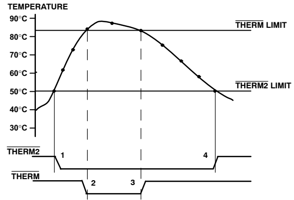
Figure 21. Operation of the \overline{\text{THERM}} and \overline{\text{THERM2}} Interrupts
